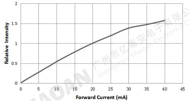
Relative Intensity VS. Forward Current (Ta=25°C)
