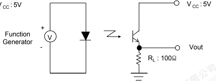
Fig 2. Test Circuit for Rise and Fall Time
