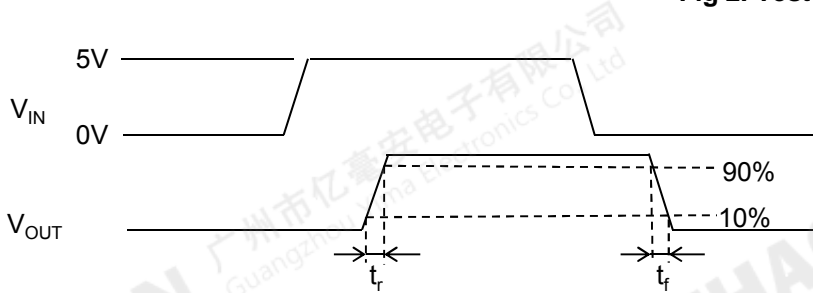
Fig 3. Definitions for Response Times
